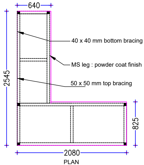
L - SHAPED CONSOLE TABLE SCHEDULE ITEM NO : 36(c)
